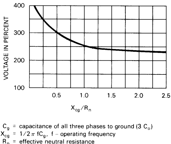
Figure 2—Transient Voltage in Percent of Rated Peak Line-to-Ground Generator Voltage for Any Number of Restrikes in the Fault Arc or Across Circuit Breaker Contacts with Distribution Transformer and Secondary Resistor Scheme of Grounding [14]
